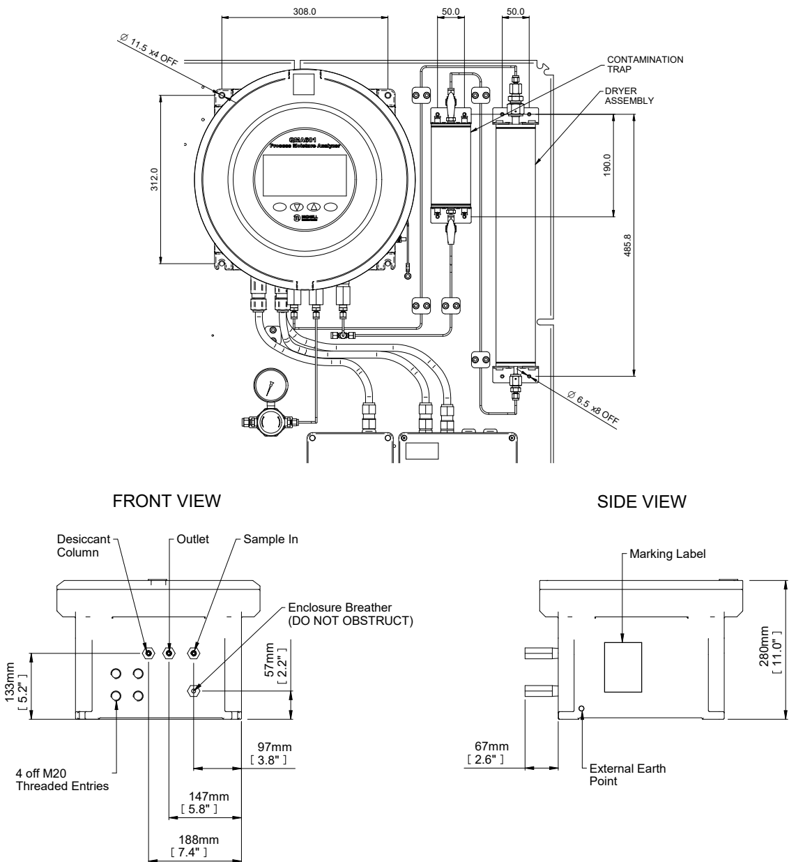
Figure 2 Mounting Dimensions
